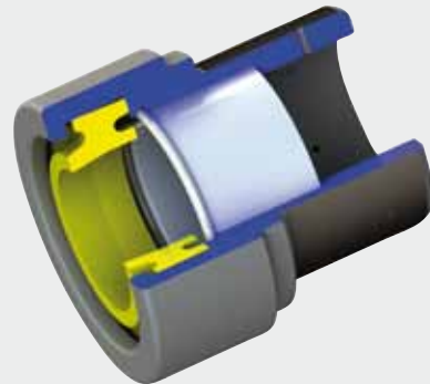
Tunnelling frontcover F-Series
