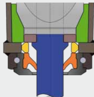
Dust protection (XS Frame)
