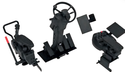
Equipped with OEM pedals, standard switches and controls, the modular system allows switching to another machine class whenever required.
