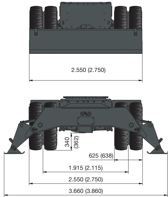
( ): Figures for 2,75 m undercarriage
